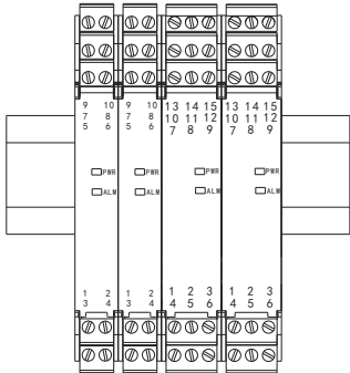
Horizontally installation
