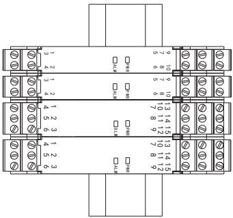
Vertically installation
