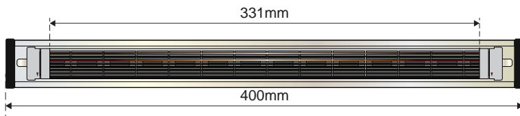
NPPB-DIN700尺寸
